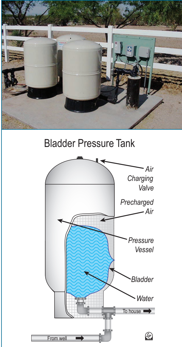
FIGURE 33. Pressure tank for a private well system. (Source: Gary Hix)
