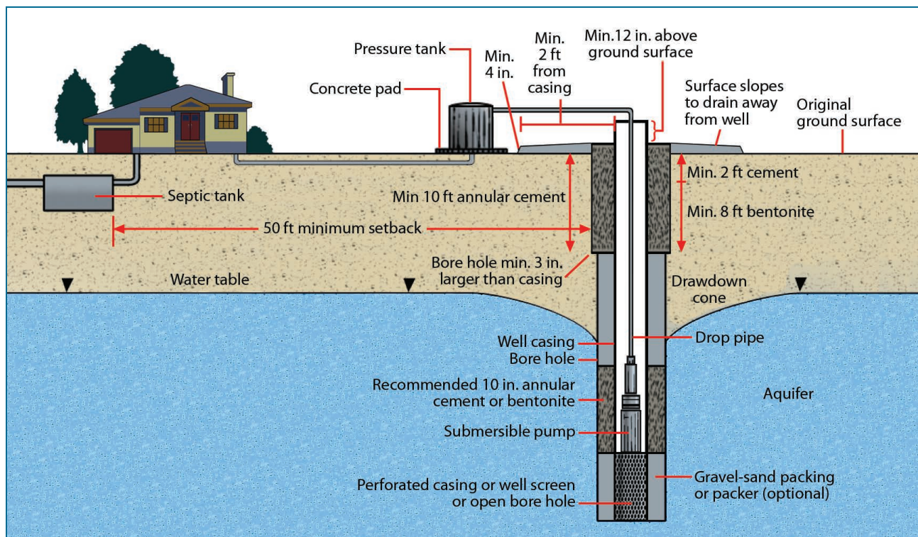
FIGURE 28. Domestic well diagram.
